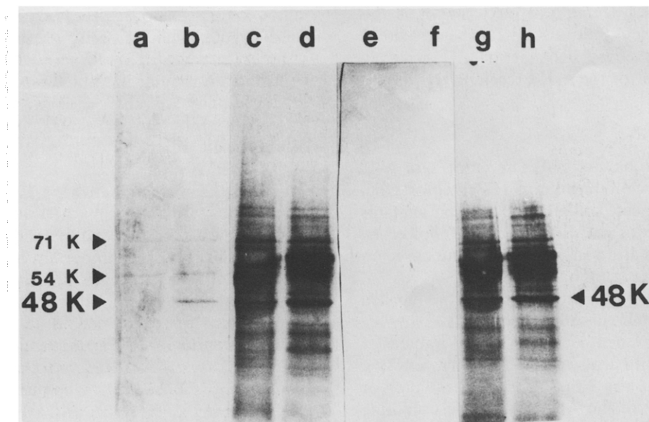
Fig.3. Western blots and autoradiographs of ^{125}\text{I} -labelled detergent solubilized EBV-transformed lymphocyte supernatants ( 100\ \mu\text{l} ) after transfer to nitrocellulose. Lanes a and b are Western blots using anti-EBNA serum of labelled detergent solubilized cell supernatants initially separated by SDS-PAGE in the absence (a) and presence (b) of mercaptoethanol. Lanes c and d are autoradiographs of a and b, respectively. Lanes e and f are Western blots using EBNA-negative serum of labelled detergent solubilized cell supernatants initially separated by SDS-PAGE in the absence (e) and presence (f) of mercaptoethanol. Lanes g and h are autoradiographs of e and f, respectively. The M_r 48000 band is indicated together with minor components M_r 54000 and M_r 71000.
